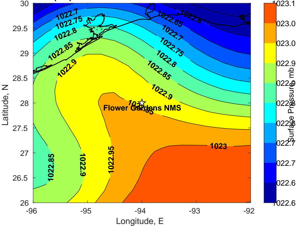
Surface Pressure (mb) for Flower Gardens NMS at 09-Dec-2020 09:00:00
